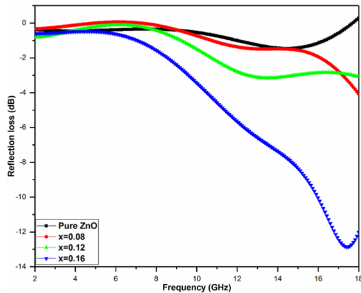
Fig. 4. Reflection loss curve as a function of frequency for ZnO/Ni composites
