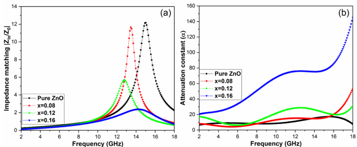
Fig. 5. (a) Impedance matching behavior at 3 mm absorber thickness and (b) attenuation constant curves as a function of frequency for ZnO/Ni composites
