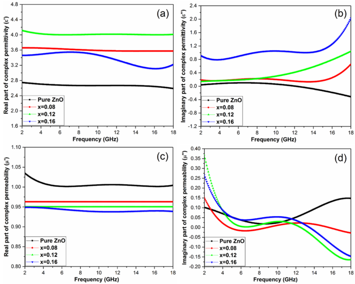
Fig. 3. (a) Real part of complex permittivity, (b) imaginary part of complex permittivity, (c) real part of complex permeability and (d) imaginary part of complex permeability with increasing frequency for ZnO/Ni composites
