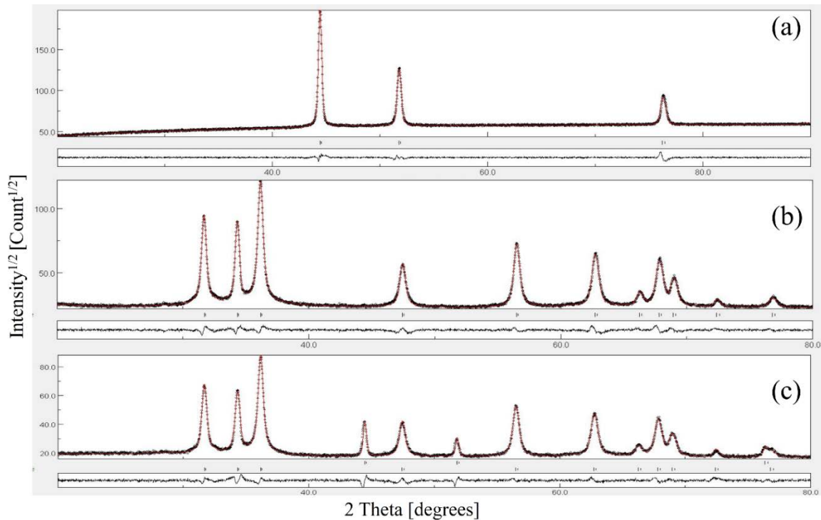
Fig. 1. Maud refined X-ray diffraction pattern for (a) Pure Ni and (b) Pure ZnO and (c) ZnO/Ni composites for x = 0.16
