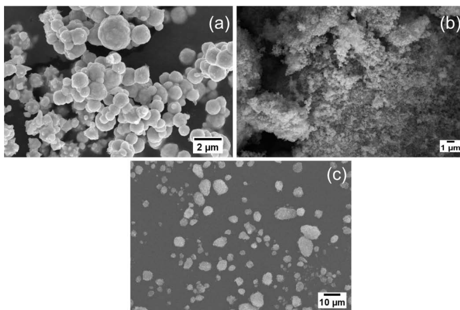
Fig. 2. SEM micrographs for (a) Pure Ni, (b) Pure ZnO and (c) ZnO/Ni composites for x = 0.16
