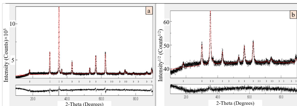
Fig. 4. Maud analysis \text{Ni}_{(1-x)}\text{Zn}_x\text{Fe}_2\text{O}_4 of ferrite for x=0.6 (a) Sol-gel (b) Hydrothermal
