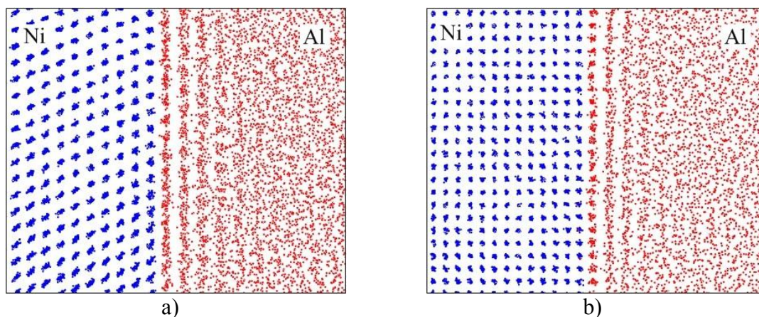
Fig. 2. Formation of a crystal structure in Al near the interphase boundary at a temperature above the melting point of aluminum (1300 K): a) (111) orientation; b) (001) orientation
