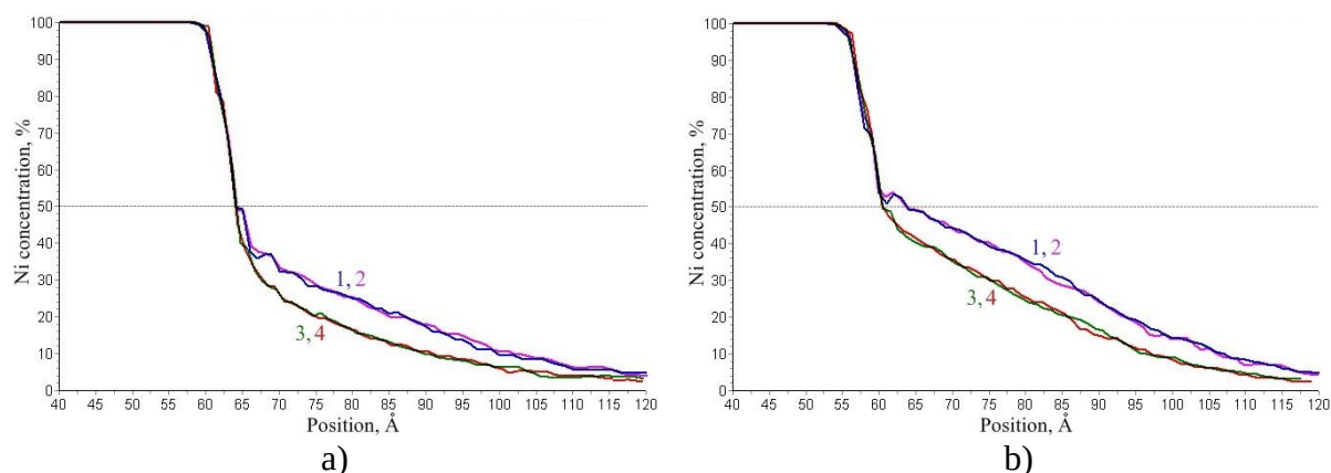
Fig. 4. Distribution of the concentration of Ni atoms in the computational cells: a) after 500 ps at a temperature of 1400 K; b) after 300 ps at a temperature of 1600 K. The numbers indicate the considered orientations: 1) (111):(111), 2) (111):(001), 3) (001):(001), 4) (001):(111)
