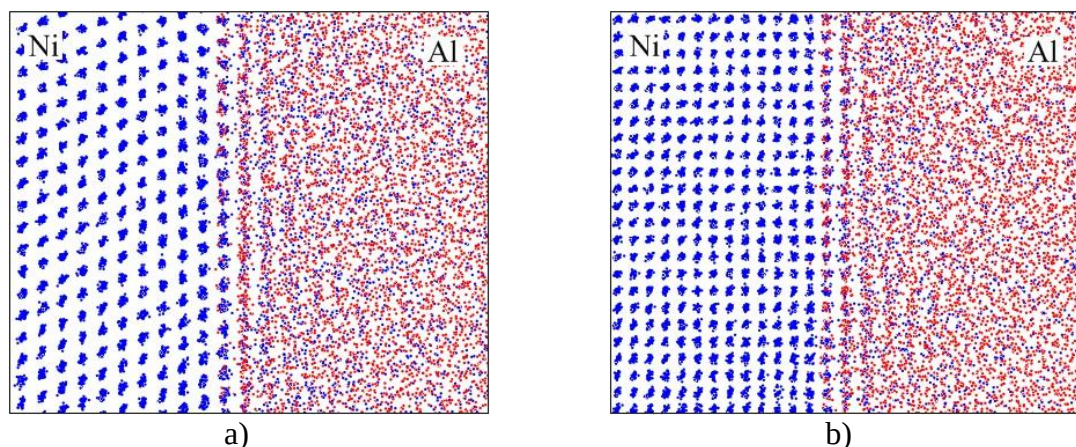
Fig. 3. Distribution of atoms in computational cells after simulation for 500 ps at a temperature of 1400 K: a) (111) orientation; b) (001) orientation
