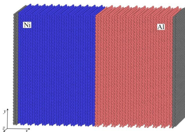
Fig. 1. Computational cell for simulating interdiffusion at the Ni-Al boundary before setting the temperature (gray atoms at the ends of the cell remained immobile during the simulation)
