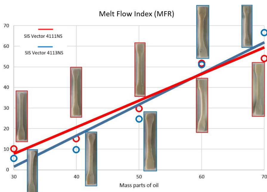
Fig. 5. MFI of compounds as a function of oil contents (for 30, 40, 50, 60, and 70 weight parts)
