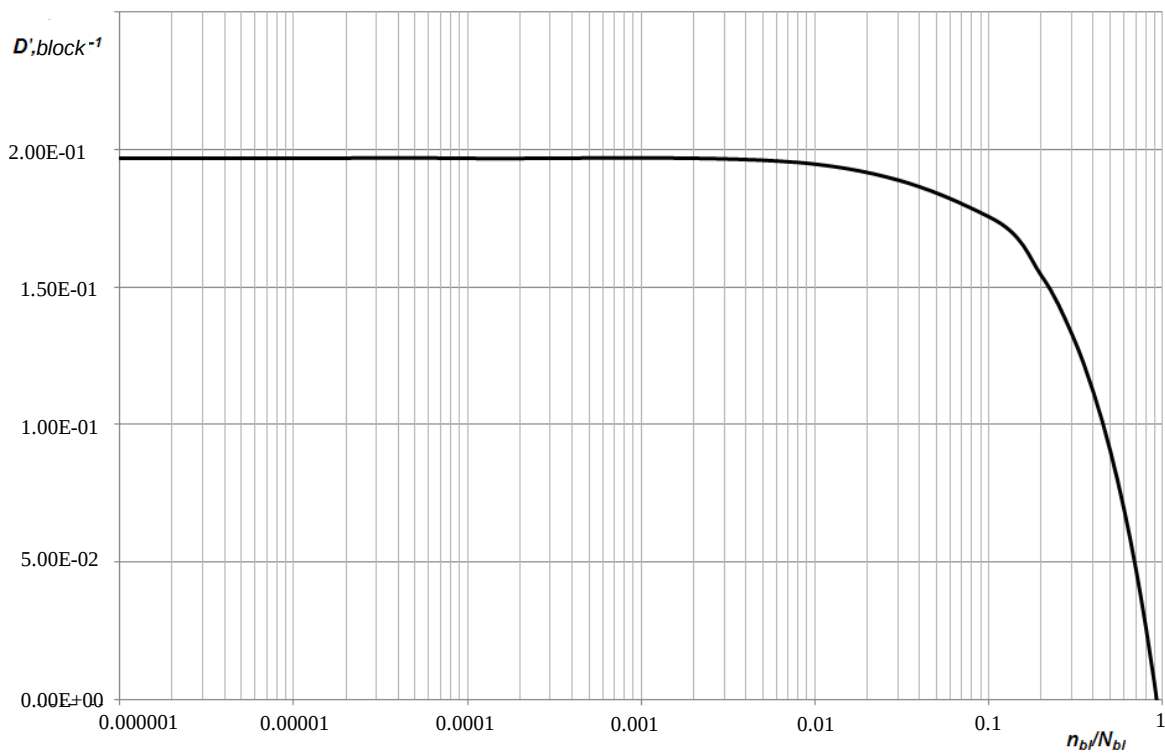
Fig. 7. Fiber splitting rate in the free-hole zone of AS4/3501-6 [0/\pm 45/90]_{s4} carbon fiber specimens
