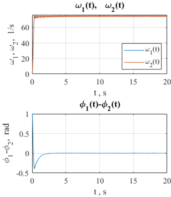
Figure 7. Simulation results for digital implementation of the control algorithm ( H^* = 75 J, \gamma_i = 0,012 , \alpha_i = 0,25 , \Delta t = 0,01 s).
