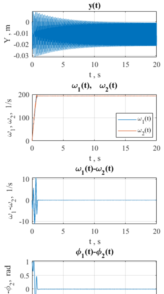
Figure 7. Simulation results for digital implementation of the control algorithm ( H^* = 75 J, \gamma_i = 0,012 , \alpha_i = 0,25 , \Delta t = 0,01 s).
