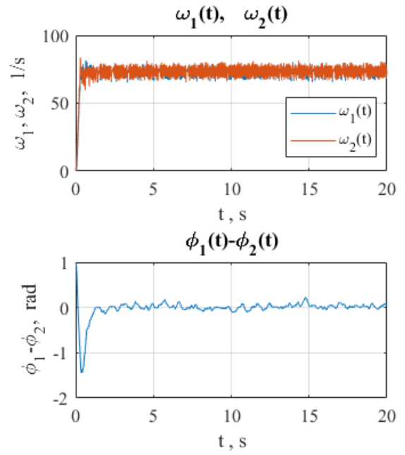
Figure 8. Simulation results for digital implementation of the control algorithm ( H^* = 75 J, \gamma_i = 0,012 , \alpha_i = 0,25 , \Delta t = 0,02 s).
