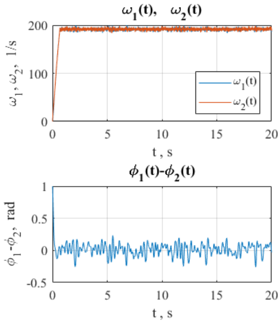
Figure 6. Simulation results for digital implementation of the control algorithm ( H^* = 500 J, \gamma_i = 0,012 , \alpha_i = 0,25 , \Delta t = 0,01 s).
