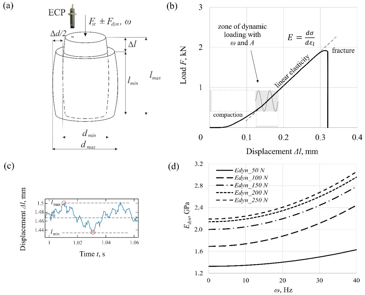
Fig. 1. Description of experiments on dynamic loading of rock samples: a) boundary shapes of the sample at maximum and minimum load (schematically); b) stress state of the sample; c) longitudinal displacement of the upper-end surface of the sample; d) dependence of the dynamic component of Young's modulus on the frequency of the applied periodic load
