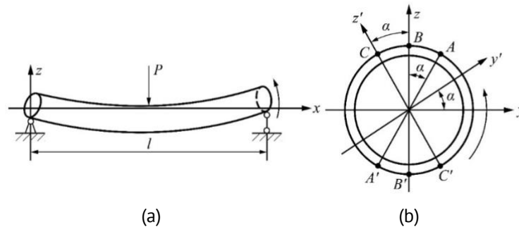
Fig. 1. Bending deformation: (a) a fixed beam; (b) a rotating beam
